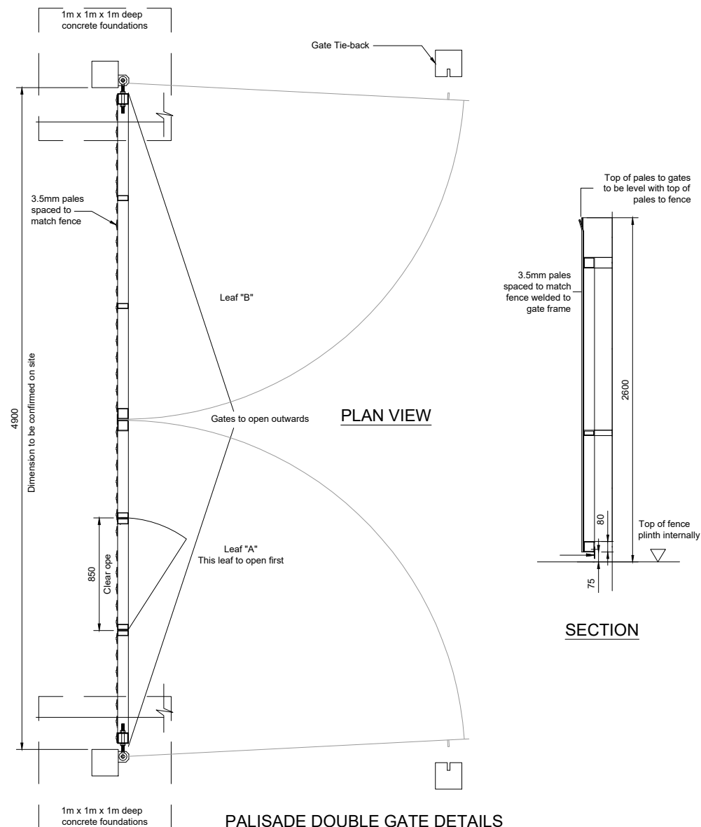
PALISADE DOUBLE GATE DETAILS
