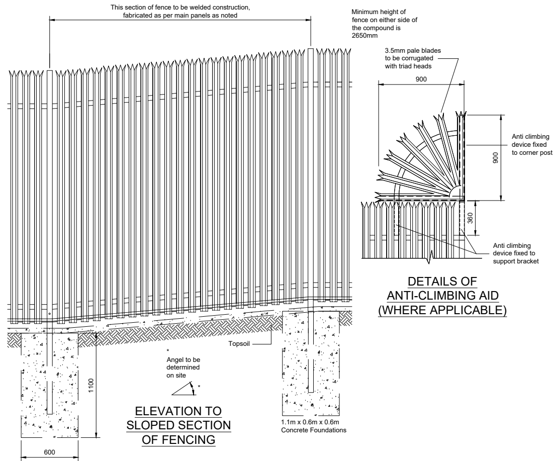
PALISADE FENCE DETAILS
